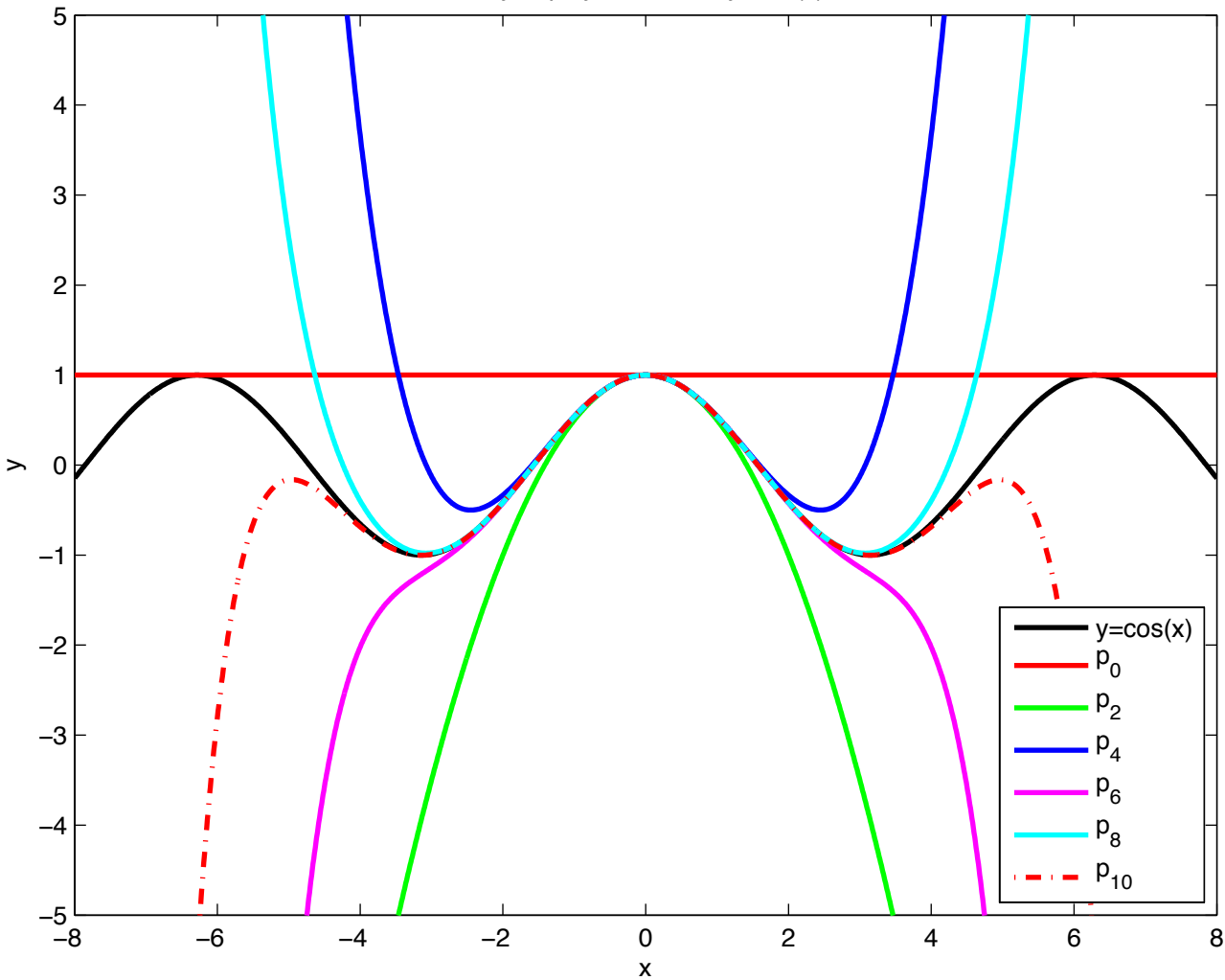
Taylor polynomials for y=\cos(x)
