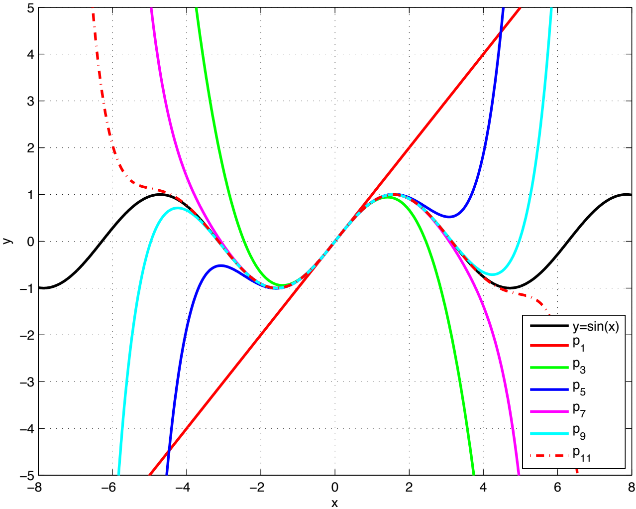
Taylor polynomials for y=\sin(x)
