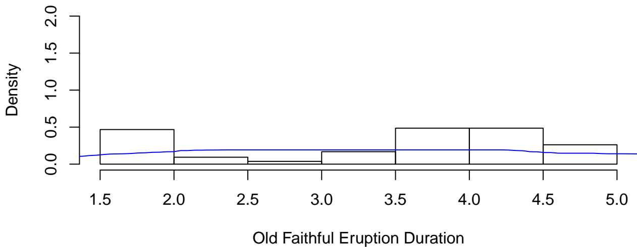
Rectangular kernel function, very large bandwidth ( \Delta = 1.5 )
