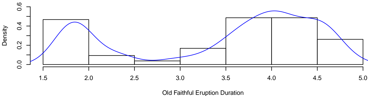
Gaussian kernel function, Sheather–Jones bandwidth rule ( \Delta = 0.185 )
