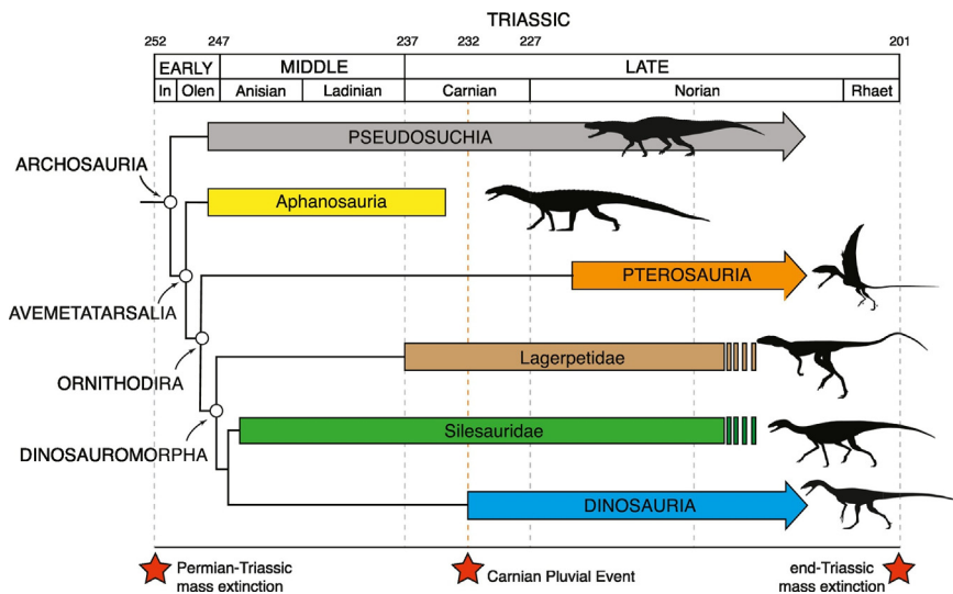
Fig. 3. Evolution of archosaurs, and evidence for early origin of dinosaurs. The oldest certain dinosaurs are mid-Carnian in age, but their sister group, the Silesauridae, date back to the Anisian, demonstrating a 15-Myr ghost range for Dinosauria. Related taxa such as Aphanosauria confirm the minimally Early Triassic origin of clade Avemetatarsalia, as well as Pterosauria and Dinosauria. Original figures kindly provided by Sterling Nesbitt.
