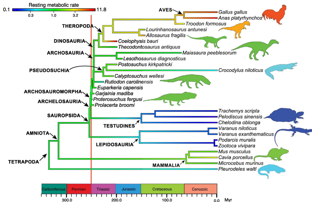
Fig. 13. The evolution of endothermy in archosauromorphs and synsids from the Permian to the present day. In the analysis, ancestral states of resting metabolic rates, measured in \text{mLO}_2\text{h}^{-1}\text{g}^{-0.67} , are estimated at each branching point in the phylogeny and colour-coded to indicate the level (note the logarithmic scale). Values for ectotherms are typically <1.0 , and for endotherms >1.0 , with modern mammals having RMR values in the range 1.5–3.5, and modern birds, 8–12 \text{mLO}_2\text{h}^{-1}\text{g}^{-0.67} . Based on data in Legendre et al. (2016), with thanks to Lucas Legendre for the base image.
