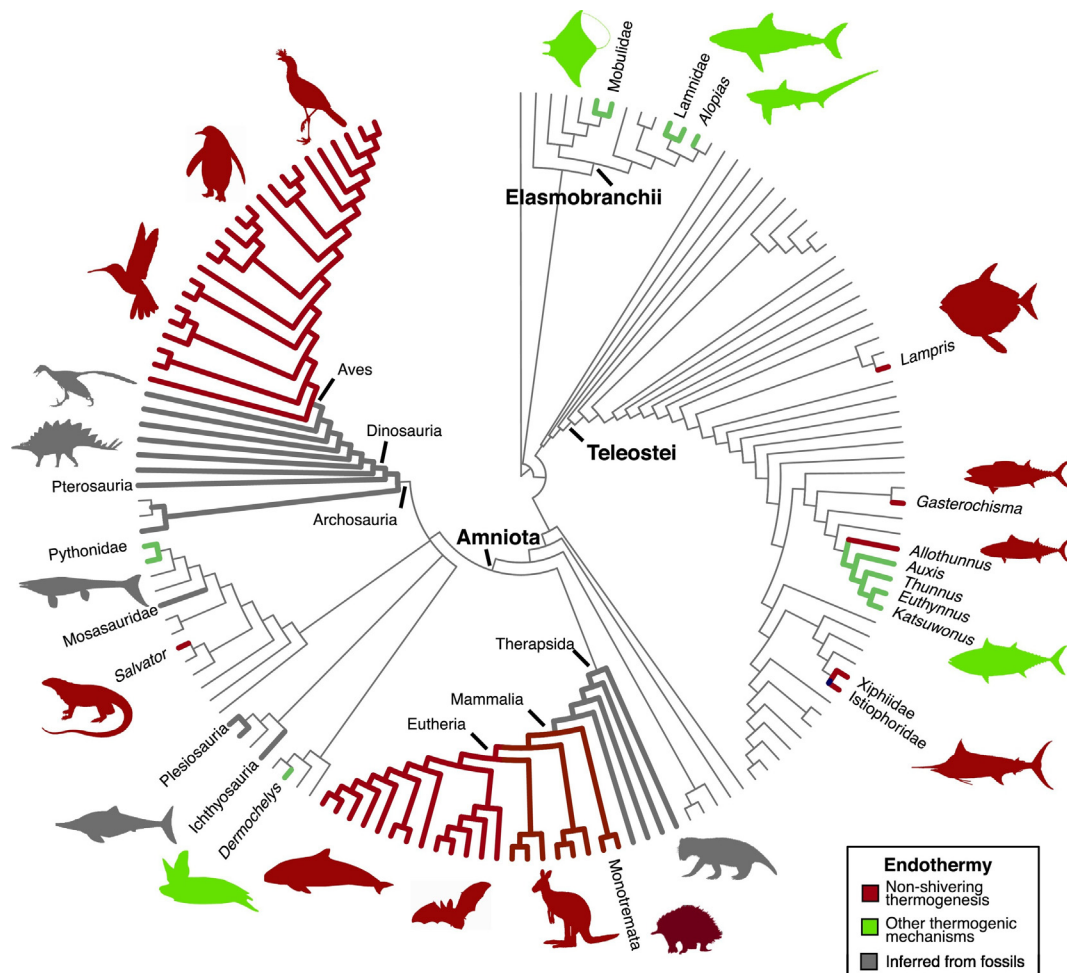
Fig. 14. Evolution of endothermy among vertebrates, showing numerous independent origins among fishes and tetrapods. Two styles of warm-bloodedness are noted: full endothermy or non-shivering thermogenesis (NST), and other strategies, including shivering thermogenesis. Thermophysiology of fossil taxa is inferred from metabolic rates calculated from four characteristics of their bone histology (see text). There are two modifications from the original, with removal of the question mark from Dermochelys as large sea turtles show NST like the various fishes, and Monotremata are shown with NST (Polymeropoulos et al., 2017). Based on data in Legendre and Davesne (2020), with thanks to Donald Davesne for the base image.
