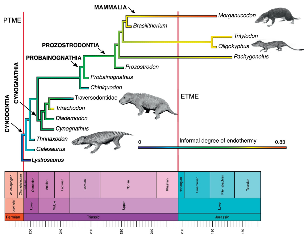
Fig. 15. Evolution of endothermy among synapsids, showing a range of values of an informal metric of endothermy (data in Table 1, see text for explanation). The small animal images are by Nobu Tamura ( Thrinaxodon , Oligokyphus , Exaeretodon ) and FunkMonk ( Morganucodon ), all Creative Commons (Wikimedia).
