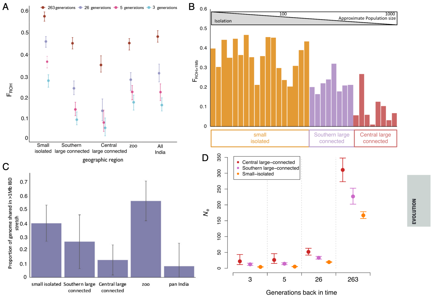
Fig. 1. Inbreeding and shared ancestry in Indian tigers. Here we show cumulative inbreeding due to parental shared ancestry due to ancestors at different historical time ranges as estimated by different lengths of ROH; that is, ROH \geq 10 Mb indicate shared ancestry on average up to 3 generations ago, 5-Mb stretches indicate on average up to 5 generations ago, 1-Mb stretches indicate on average up to 26 generations ago, and 0.1-Mb stretches indicate on average up to 263 generations ago. Shown is the cumulative inbreeding in each population due to shared ancestry between parents at each time range. Error bars are 95% CI. (A) Inbreeding in individuals due to shared ancestry 26 generation ago. (B) The proportion of the genome shared in 1-Mb or longer tracts between pairs of individuals from a population of individuals belonging to central large-connected, southern large-connected, and small-isolated populations. Pan-India comparisons in C include all pairwise comparisons of wild individuals. Error bars are SEs. N_e over time is estimated from F_{ROH} for the different populations. (D) Error bars are SDs.
