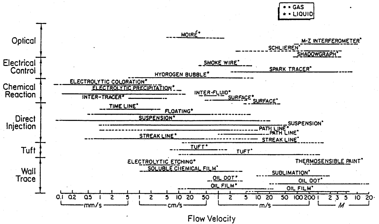
Fig. 2 Applicable flow range for each flow visualization method.
