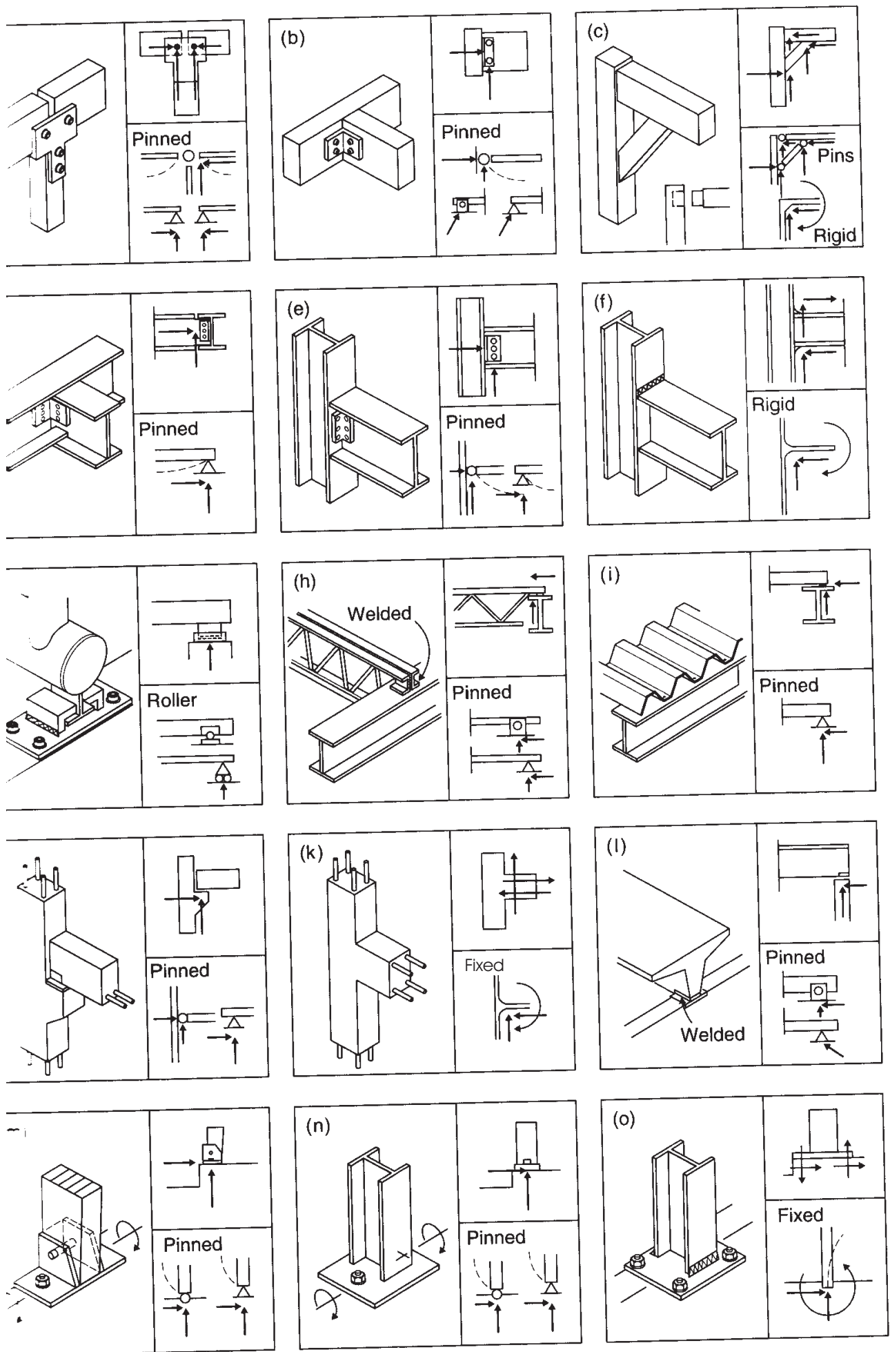
FIGURE 3-8 Types of connections and idealized models.
