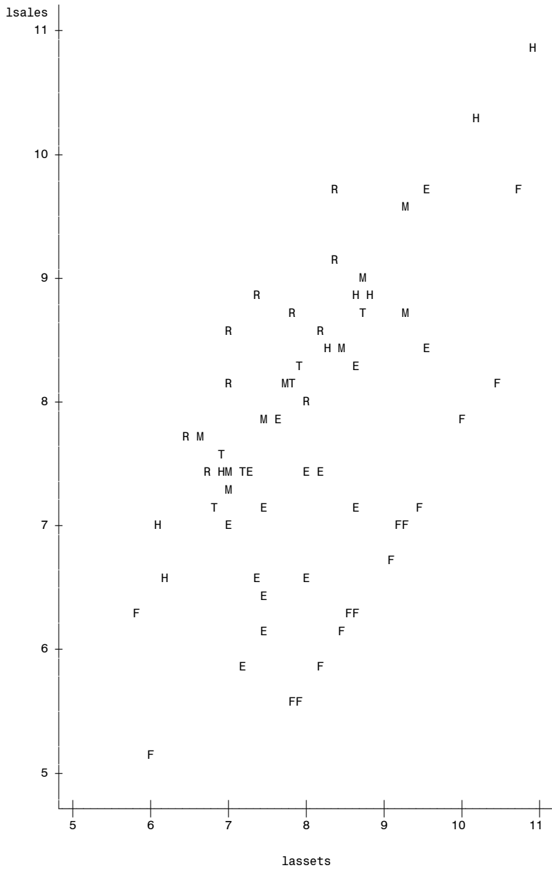
Plot of lsales*lassets. Symbol is value of sect.
