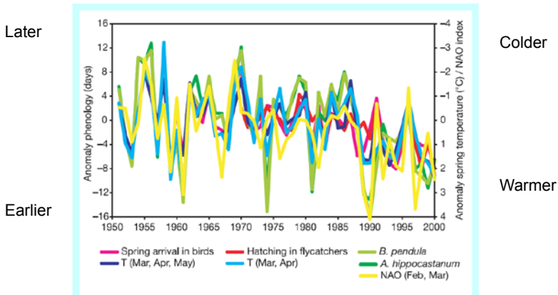
Figure 2 Anomalies of different phenological phases in Germany correlate well with anomalies of mean spring air temperature T and NAO index (by P. D. Jones, http://www.cru.uea.ac.uk/cru/data/nao.htm ). Temperature taken from 35 German climate stations. Phenological phases used: spring arrival in birds, island of Helgoland, North Sea; hatching in flycatchers ( Ficedula hypoleuca ), Northern Germany; and mean onset of leaf unfolding of Aesculus hippocastanum and Betula pendula .
