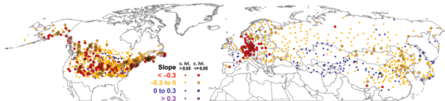
Fig. 1 Spring indices (SI) first leaf date 1961–2000 trend by station. Trend values are in days per year. Stations with trends significant at the 0.05 level or better are shown with larger symbols (Sagarin, 2001).
