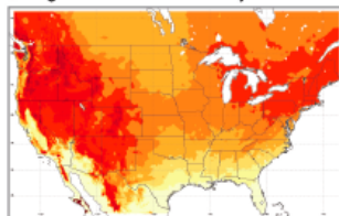
Change in Number of Frost Days
