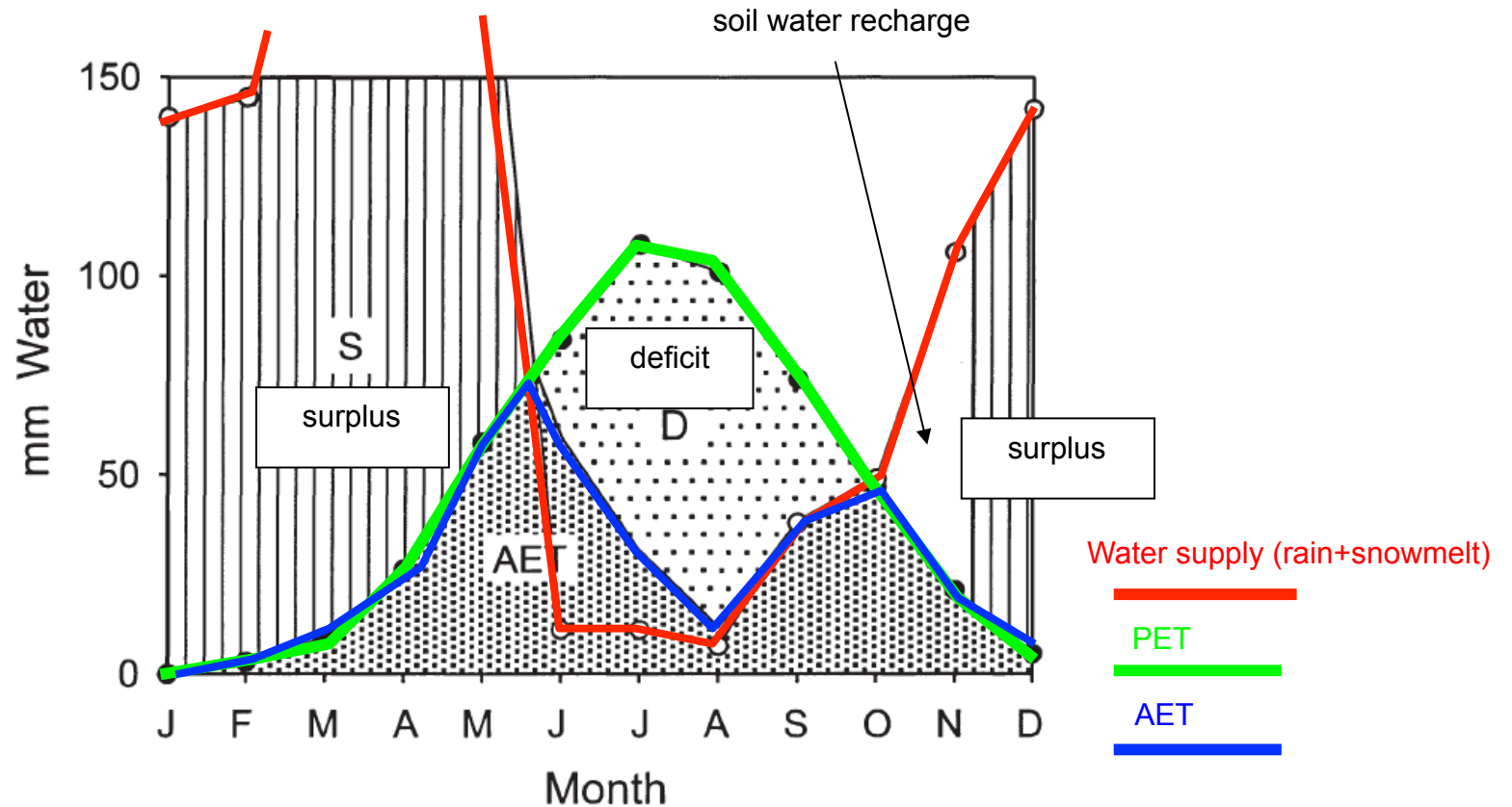
FIG. 1. The annual water balance of a site on level ground, soils of 0.5 m depth, at 2000 m elevation, and in the wet Kaweah watershed of the southern Sierra Nevada (data from Stephenson, 1988). From October through May, water supply (rain plus snowmelt, \circ ) exceeds evaporative demand (potential evapotranspiration or PET, \bullet ); during this period, actual evapotranspiration (AET, dense stippling ) equals PET. In October and November, excess water replaces soil water used during the summer; the white area between the water supply and PET curves represents soil-water recharge. From November through May, after soil water has been replenished, the difference between water supply and PET is surplus (S, vertical stripes ). From June through September, PET exceeds water supply. During this period, AET equals water supply plus water extracted from the soil (which is shown as the curve between the water supply and PET curves). Deficit (D, light stippling ) is the difference between PET and AET.
