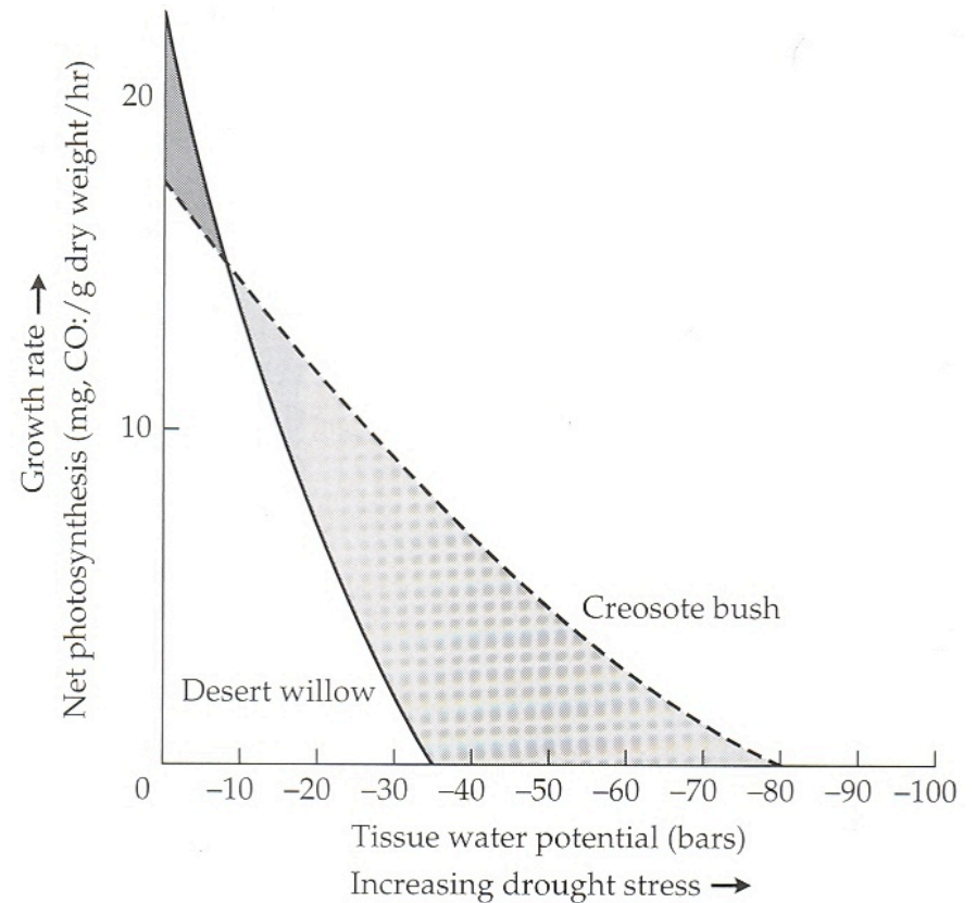
FIGURE 4.23 Trade-offs between growth rate and drought tolerance in two species of desert shrubs: creosote bush ( Larrea tridentate ), which grows in some of the driest North American deserts; and desert willow ( Chilopsis linearis ), which has an overlapping geographic range, but is more mesophytic, occurring in microhabitats along watercourses where the soil is permanently moist. Note that under relatively high drought stress (light gray region) creosote bush has the higher net photosynthetic rate and is able to grow faster, shade, and competitively exclude desert willow. (After Odening et al. 1974.)
