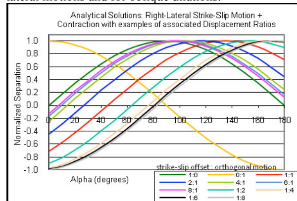
Figure 1. Plots of various analytical solutions have been created to compare against measured results to best determine the DR (strike-slip offset:orthogonal motion) for each ridge or band investigated.
