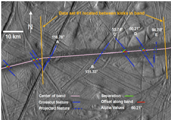
Figure 2. An unnamed band in Galileo image s0449961865r (23.1°N, 221.6°W). Crosscut features are shown in blue, projected features (blue dashed lines), offsets are shown in red and separations are shown in green. Resolution is ~220 m/pix.
