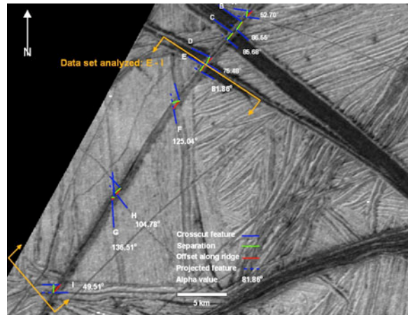
Figure 4. An unnamed ridge is shown here in the Argadnel Regio region (Galileo image number s0426273839r). Features are labeled using the same color scheme as in Fig. 2. Image resolution is ~50 m/pix.
