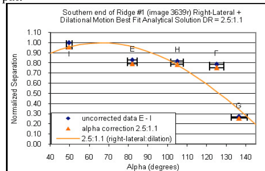
Figure 5. This graph illustrates a relatively good correlation (SCR of 0.65) between the normalized data set and the analytical solution of a DR of 2.5:1.1.
