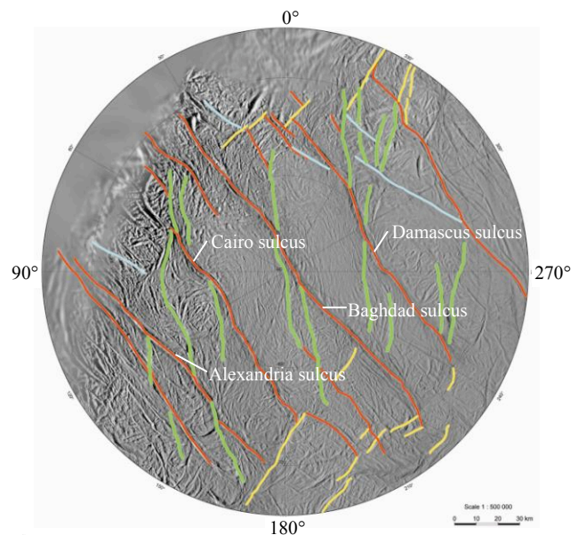
Figure 1: Polar projection of the South Polar Terrain on Enceladus. The scale bar is 30 km. Fractures show a progressive rotation of fracture orientations. From youngest to oldest, the fracture sets are believed to proceed from red, which include the tiger stripes, blue, green, and the oldest in yellow. Mosaic is from [9].
