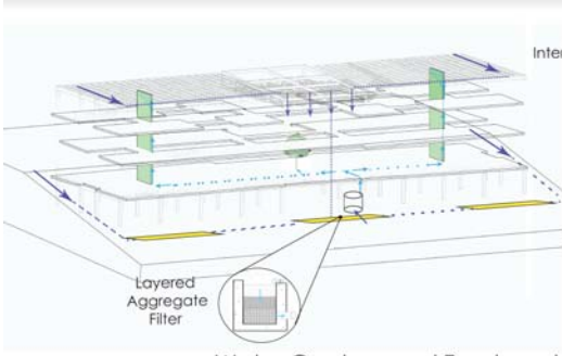
Water Capture and Treatment
