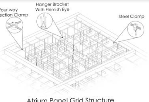
Atrium Panel Grid Structure
