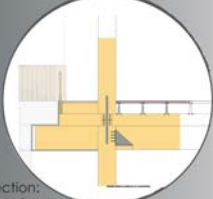
Wall Section: Southern Overhang
