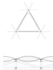
Tri-grid Pillows ETFE Panel Options
