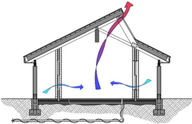
McCall Outdoor Science School Ventilation Diagram
