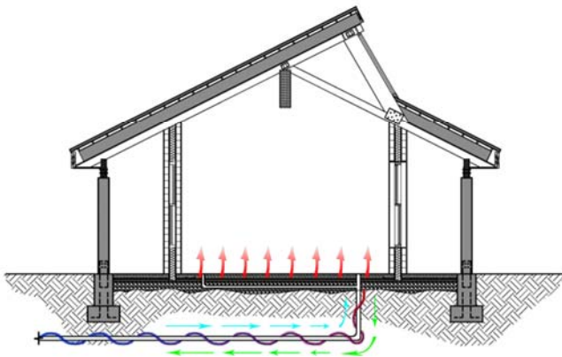
McCall Outdoor Science School Plumbing & Geothermal Diagram
