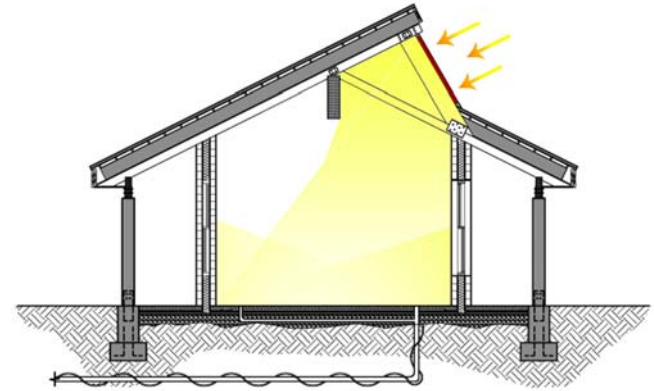
McCall Outdoor Science School Sun Diagram
